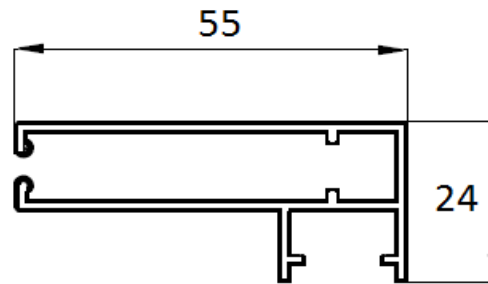
Coulisse occultante OC pose de face:
